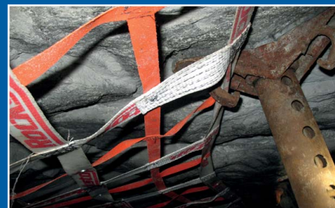
Rockstop attached to temporary support
