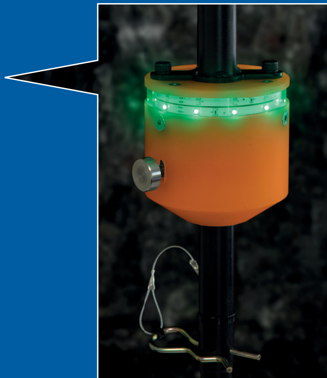
Green flashing LED lights indicate a safe working environment Red flashing LED lights indicate separation in the strata above
